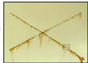
COMMON COLD ROLLED SHEET STEEL with a 1 mil dry film build paint thickness after a 336 hour salt spray test.
