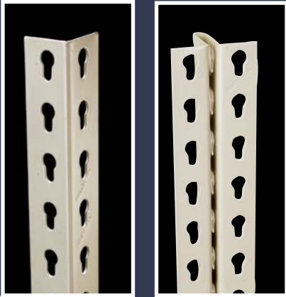
1 Angle Post 2 T-Post
